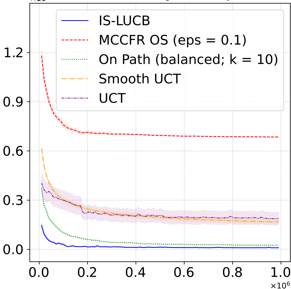
\times 10^{-1} Leduc Poker, Best Algorithms, Player o
